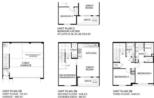
TESORO SQUARE | PLAN 2B
